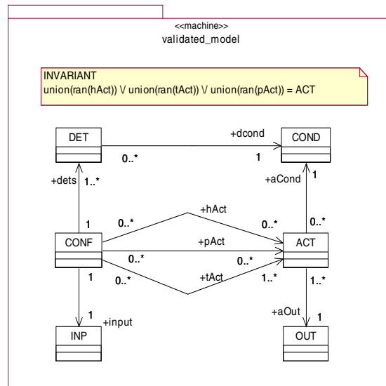
Fig. 5. Final UML-B version of generic model of failure management requirements
