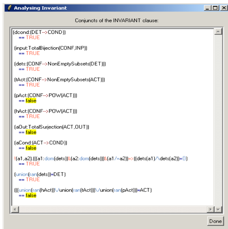
Fig. 7. ProB being used to verify the example application
